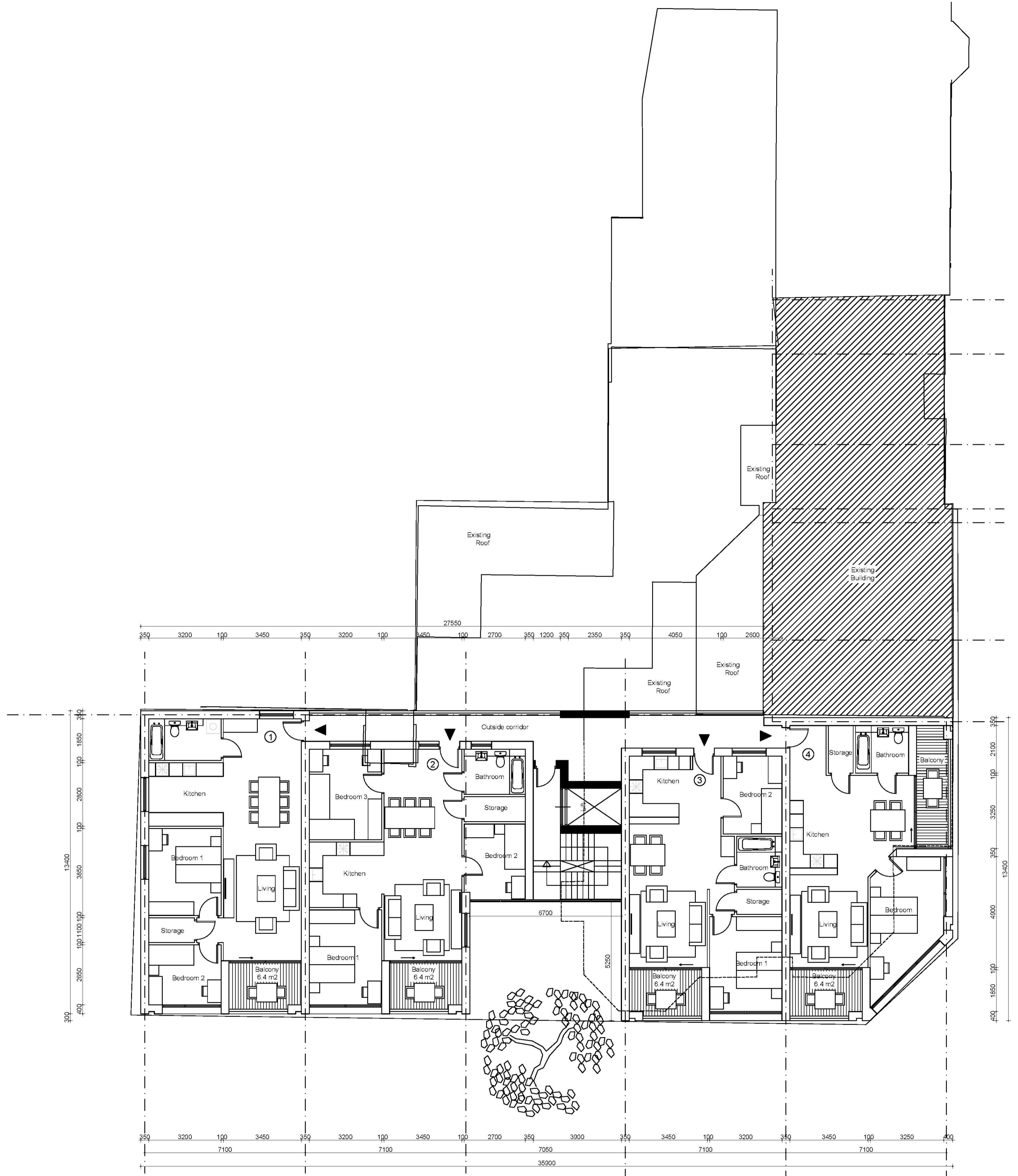
Proposed 1st Floor Plan
